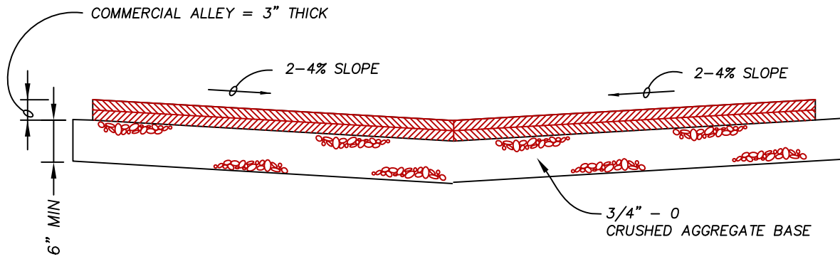
TYPICAL ALLEY (INVERTED CROWN) SECTION
