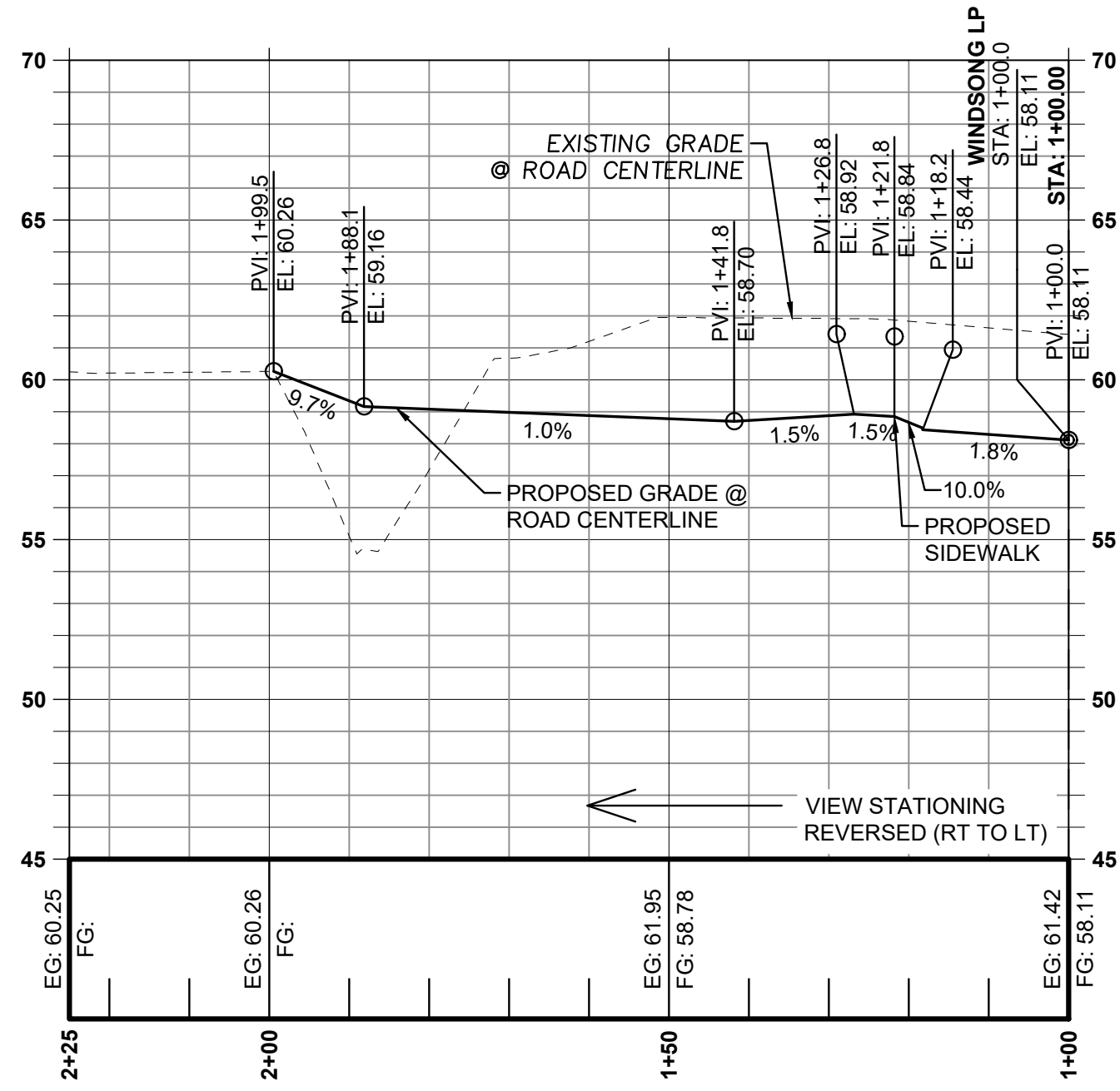
AUTUMN GOLD LN PROFILE (STA: 1+00 - STA: 2+25)
