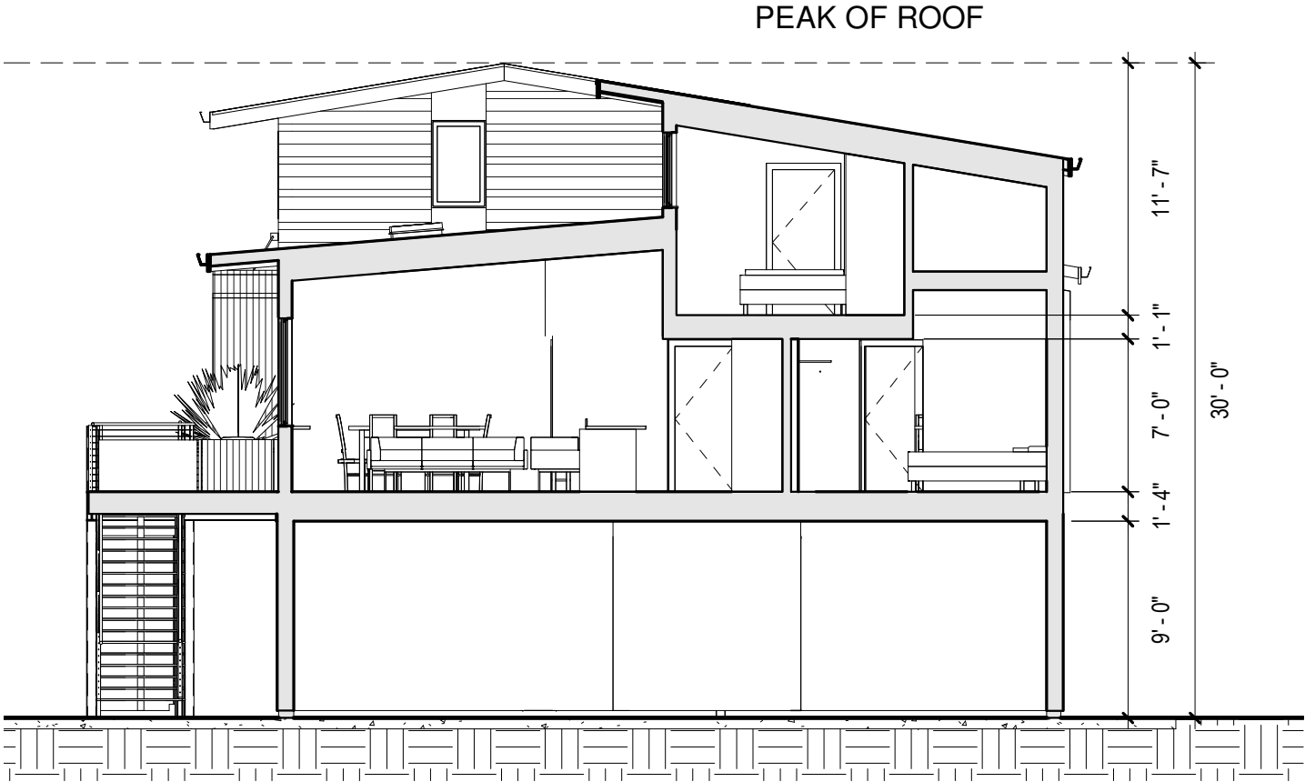
SECTION LOOKING WEST UNIT 1
