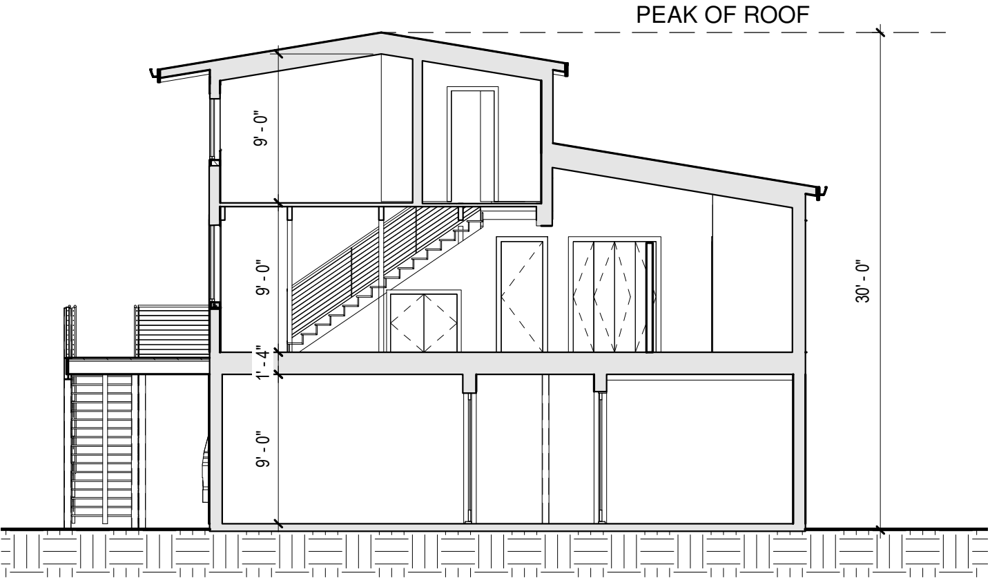
SECTION LOOKING WEST UNIT 2
