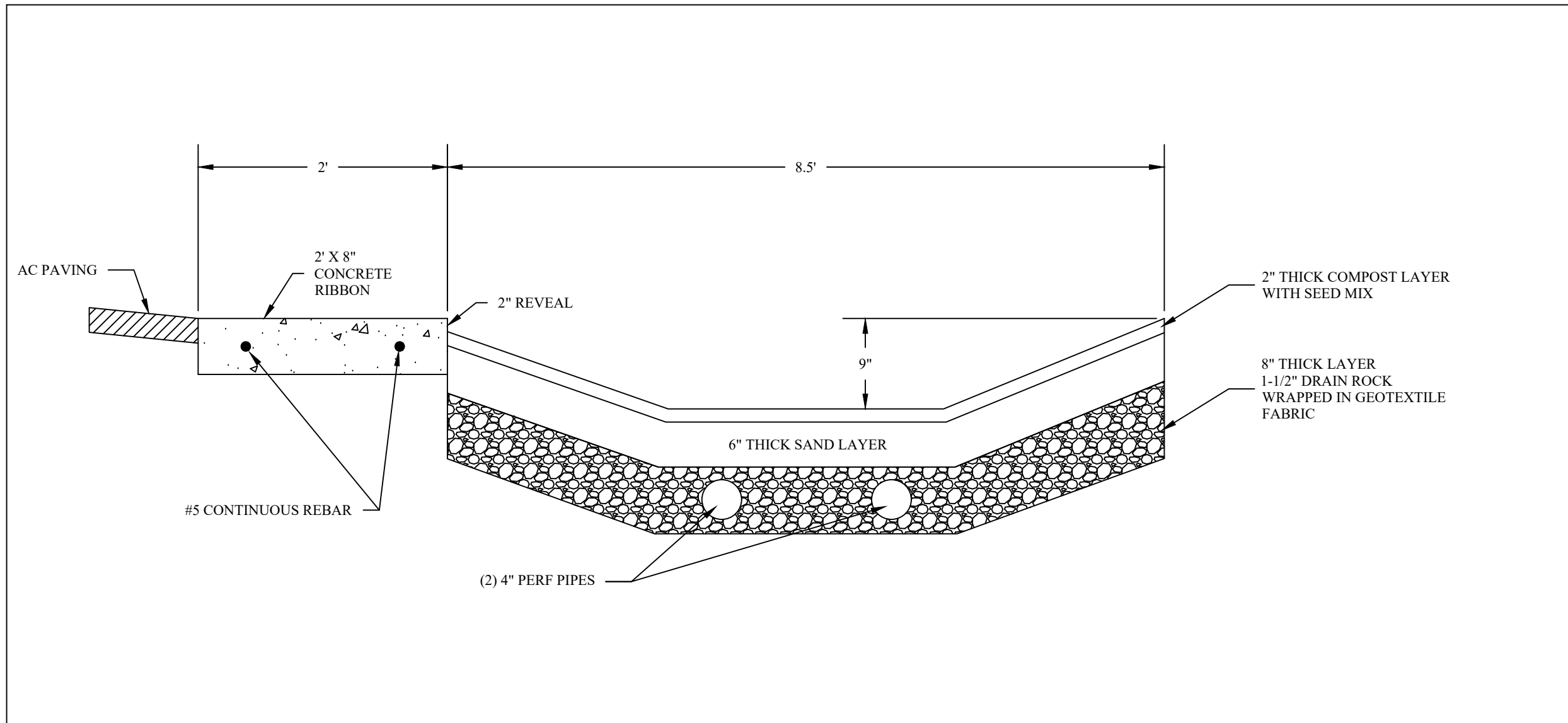
3 TYPICAL VEGETATED SWALE NOT TO SCALE
