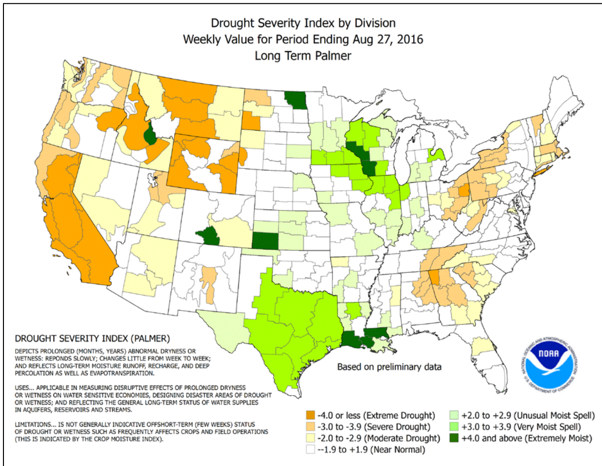
Figure 3-3 Drought Severity Index, August 2016
