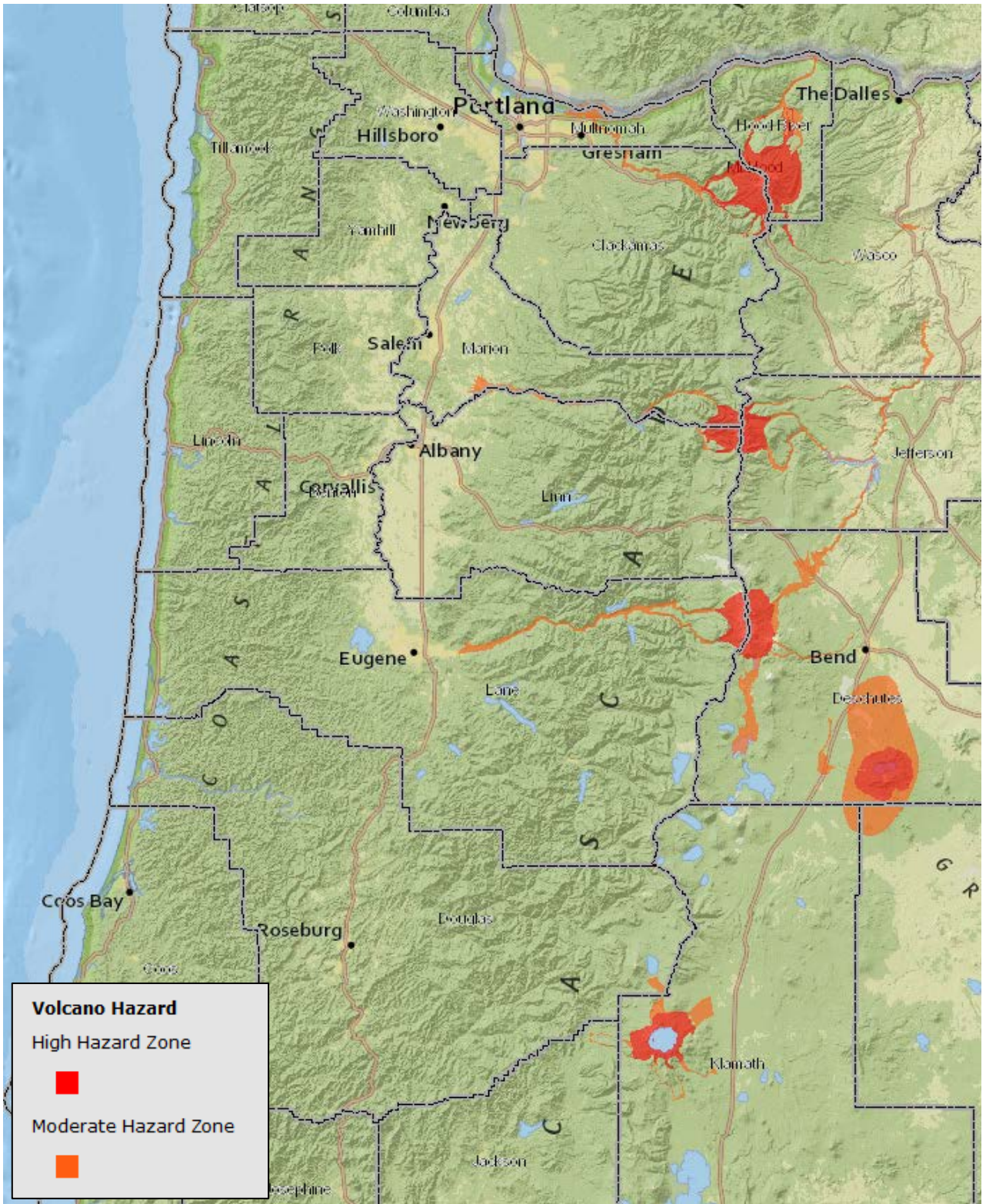
Figure 3-32 Volcanic Hazard, Western-Central Oregon (2015)
