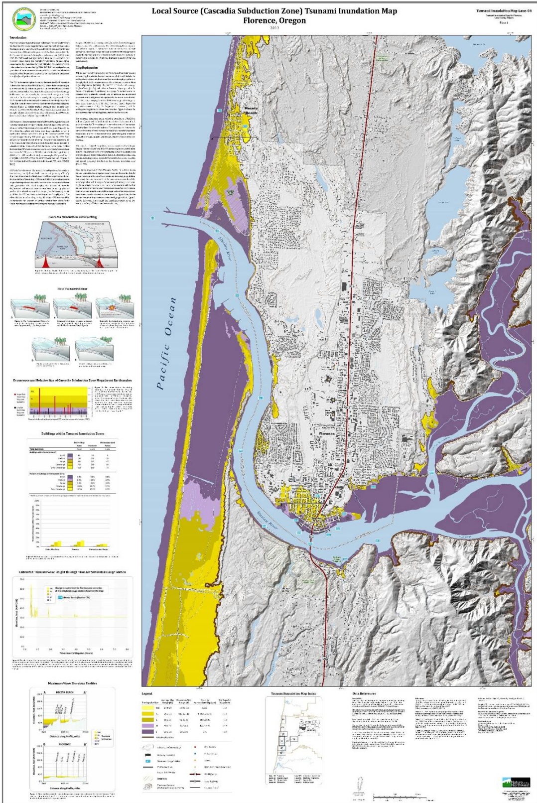
Figure 3-21 Tsunami Inundation Map: Florence, Oregon
