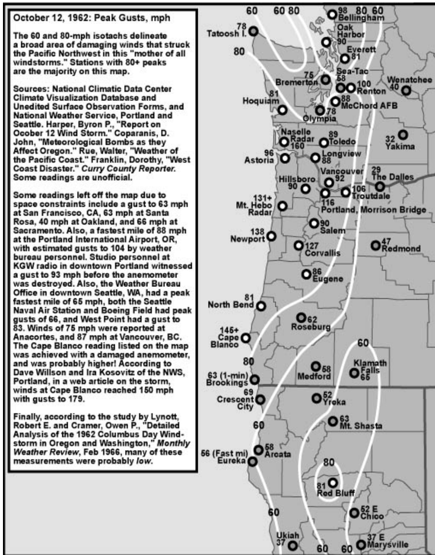
Figure 3-27 Peak Gusts, October 12, 1962 (Columbus Day Storm)
