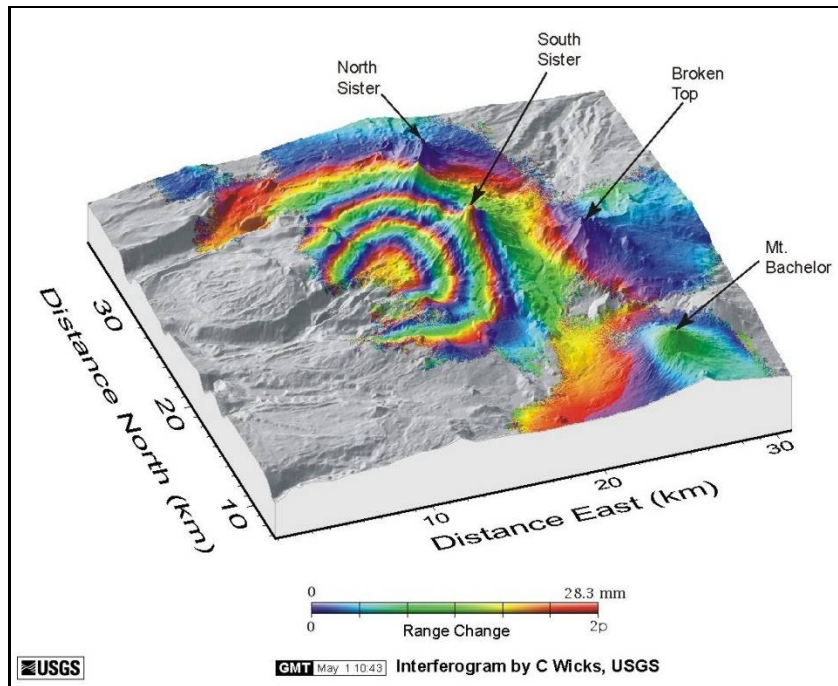
Figure 3-33 Uplift in West Three Sisters Area
