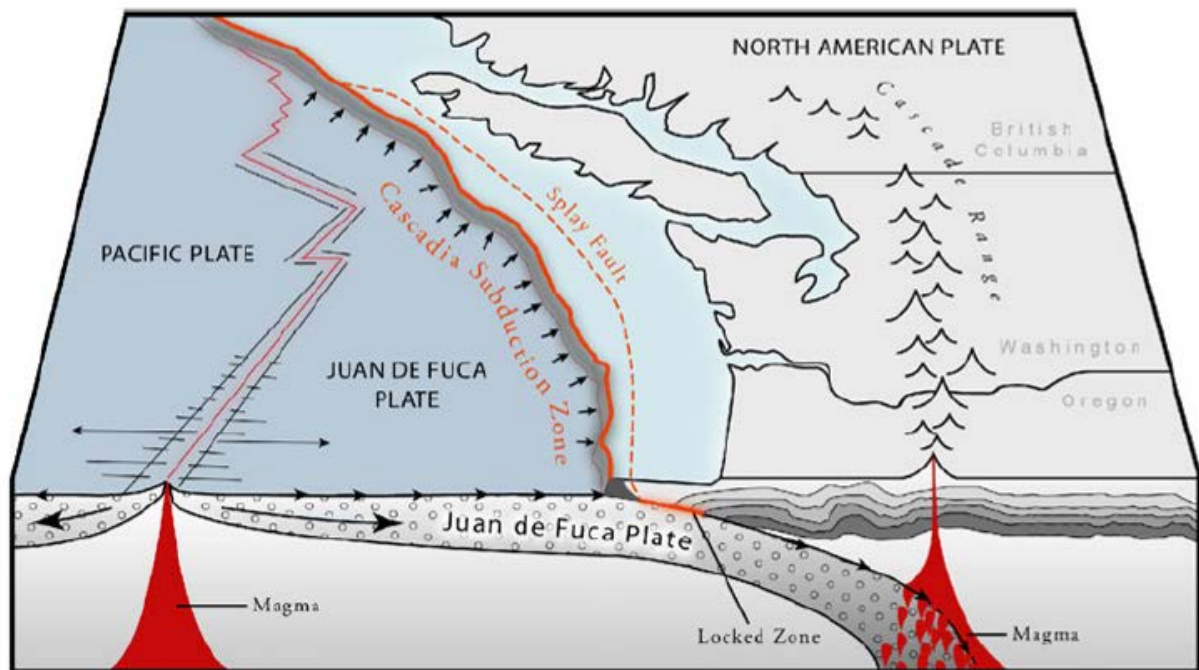
Figure 3-20 Cascadia Subduction Zone Setting
