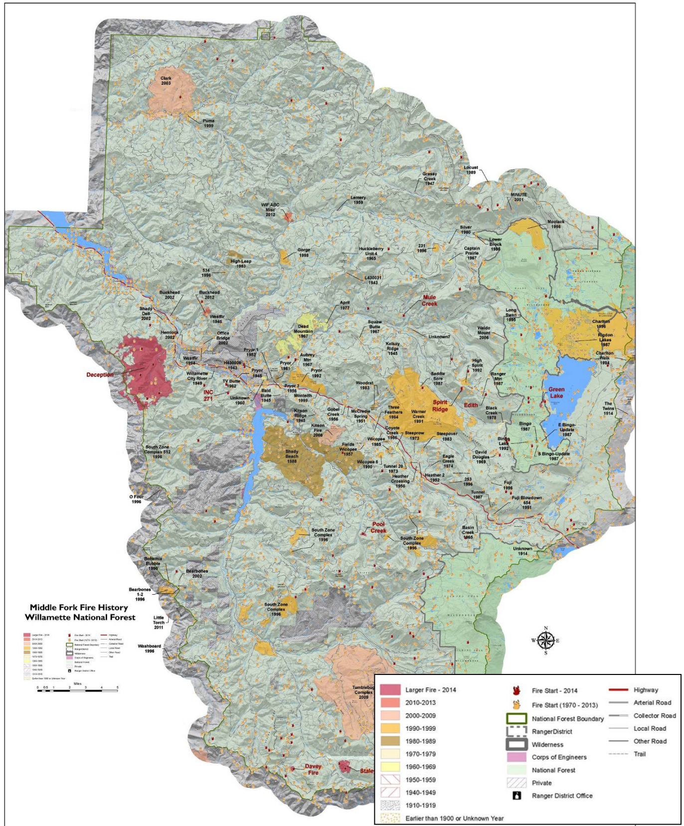
Figure 3-24 Fire History: Middle Fork Willamette National Forest
