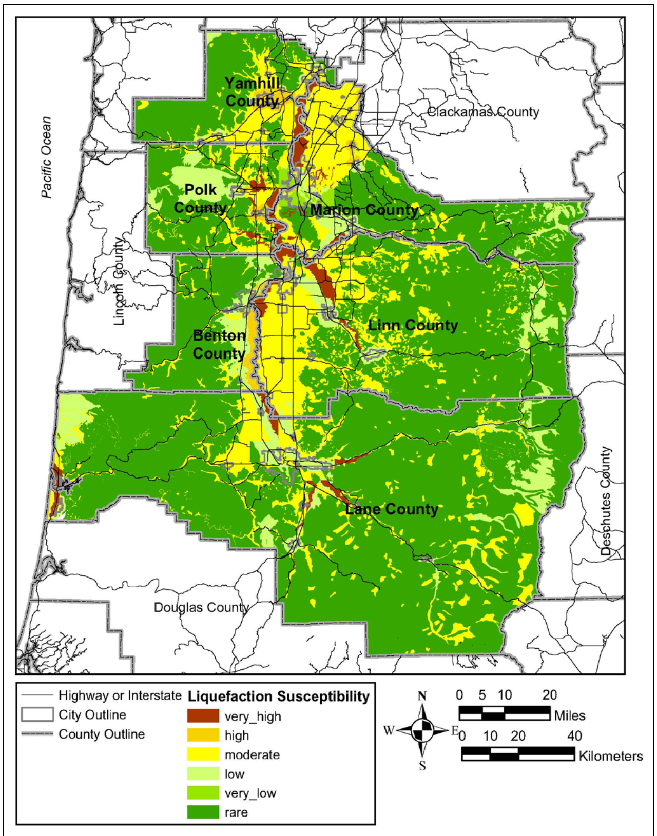
Figure 3-9 DOGAMI IMS-24 Report, Liquefaction Susceptibility, Central-Western Oregon
