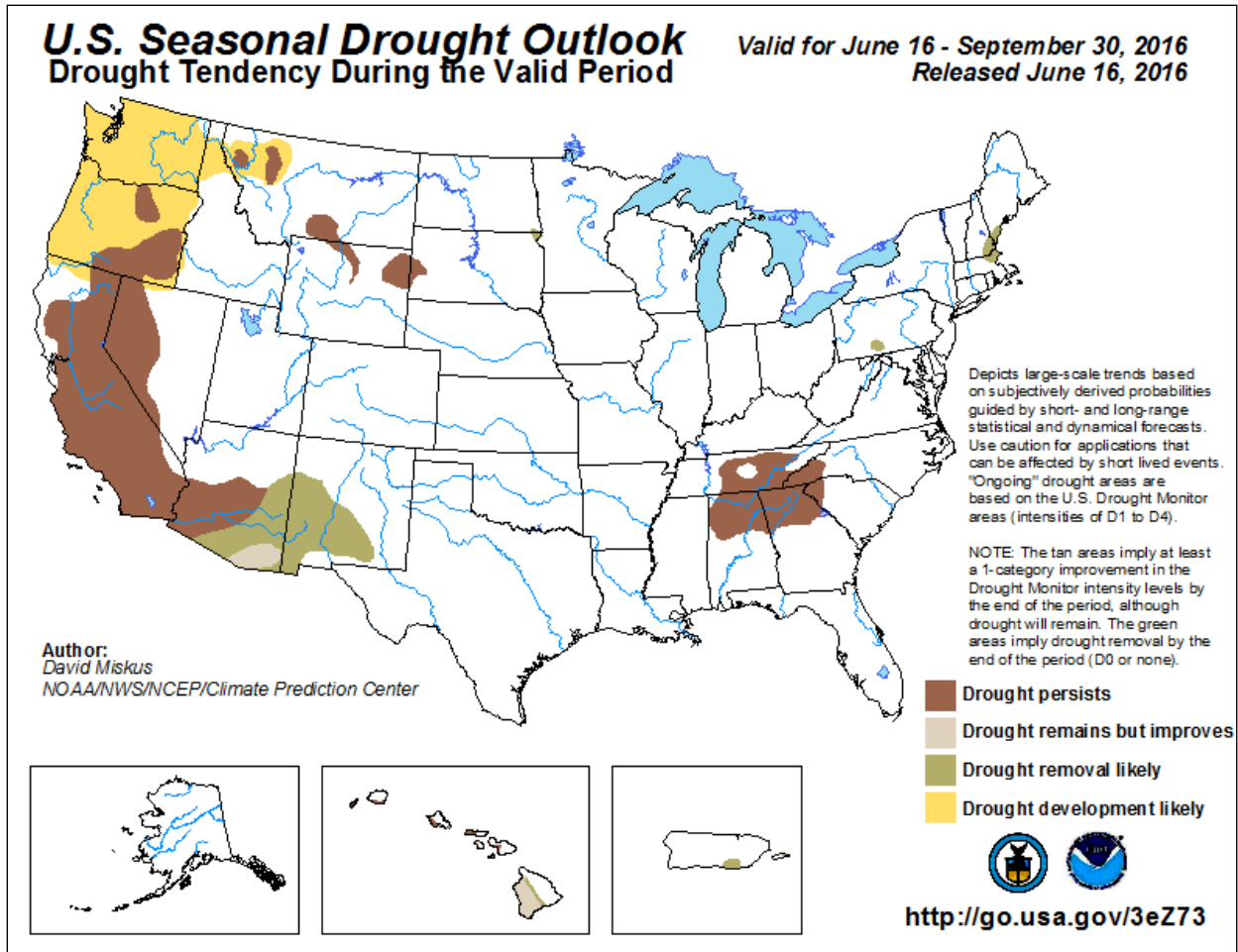
Figure 3-2 US Drought Forecast
