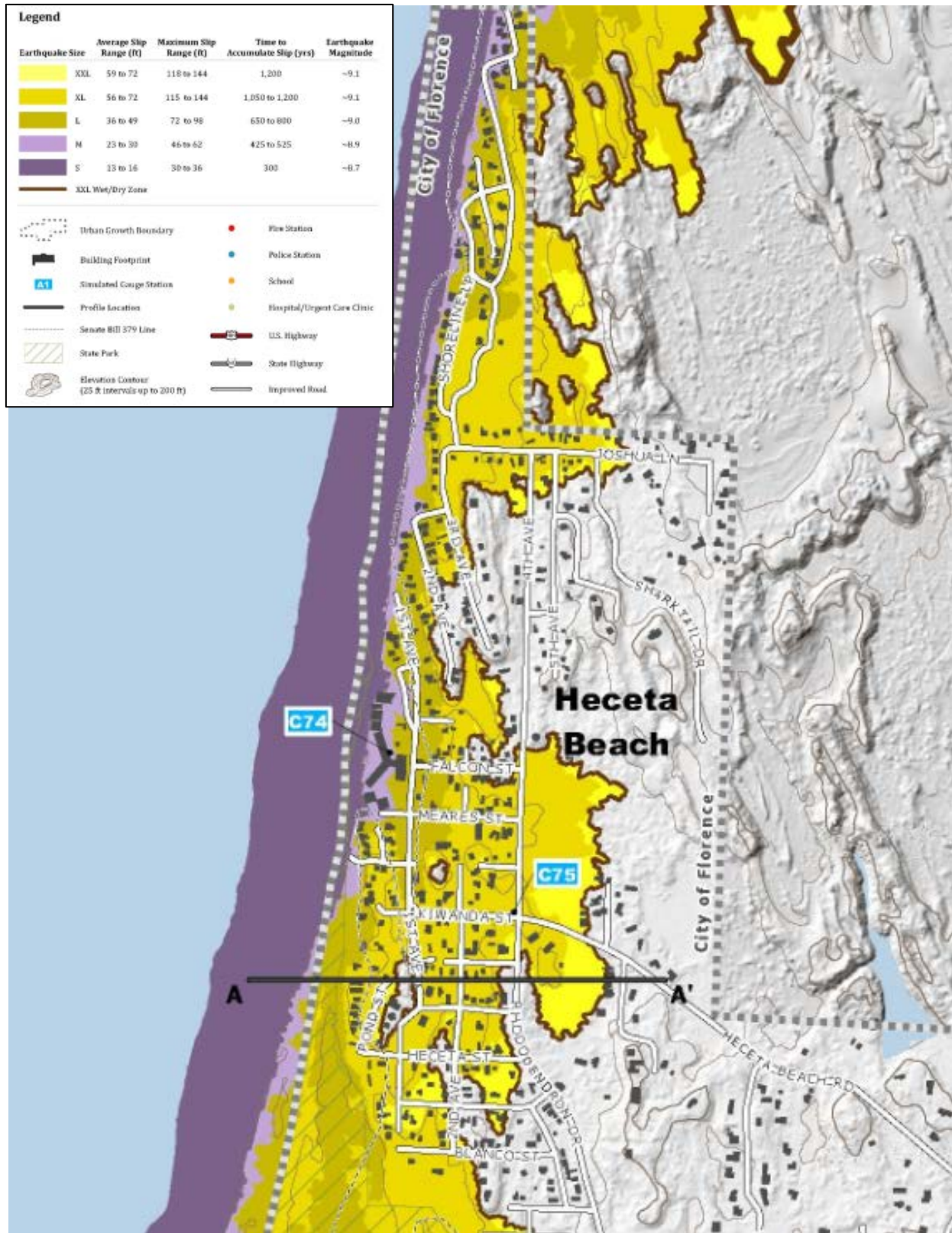
Figure 3-36 Excerpt from DOGAMI TIMs (Northwest Florence, Heceta Beach Area)
