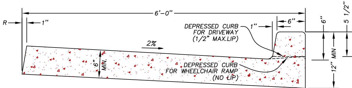
TYPICAL WIDE CURB & GUTTER
