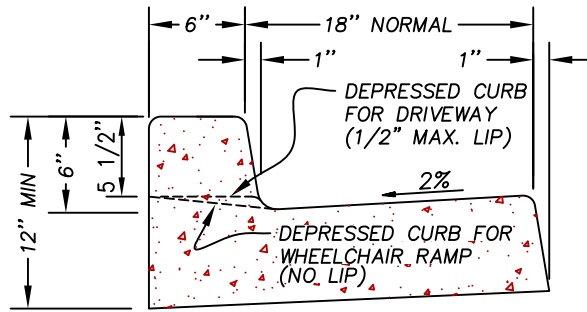
TYPICAL STANDARD CURB & GUTTER
